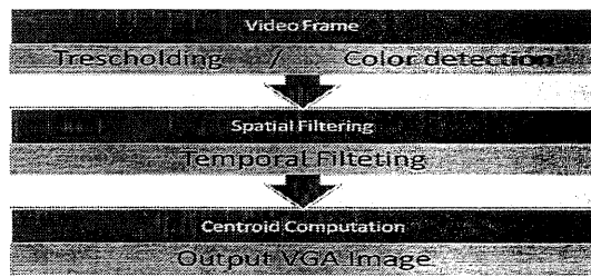
Fig.4. Hardware algorithm.
